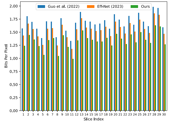
Fig. 5. A detailed comparison of the Bits Per Pixel (BPP) for each of the 30 slices in the out-of-distribution TGCT dataset. The results demonstrate that our method consistently outperforms other methods by achieving a lower bitrate for every slice.
