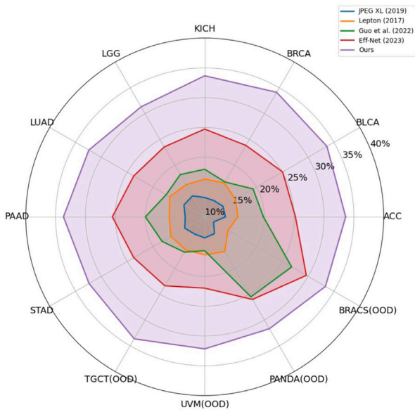
Fig. 4. Comparison of compression saving (%) on in-distribution and out-of-distribution (OOD) datasets. Our proposed method consistently outperforms all competing methods.
