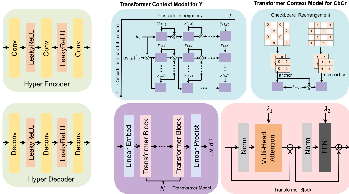
Fig. 1. Overview of the Proposed Universe Pathology JPEG Lossless Recompression Foundation Model. For the luma (Y) and chroma (Cb and Cr) components, each component comprises a hyper-network and a Transformer-based context model. The hyper-network extracts side information to learn global correlation priors, while the Transformer context model establishes long-range dependencies among coefficients to capture fine-grained local details and further reduce redundancy. The primary workflow proceeds as follows: the hyper-network encodes the DCT coefficients and quantizes them into \tilde{z} , which is subsequently compressed into a bitstream using an Arithmetic Encoder (AE). Subsequently, an Arithmetic Decoder (AD) decompresses the bitstream and generates the side information h . The Transformer context model exploits the obtained side information to estimate the entropy of each DCT coefficient, and then performs lossless compression of the DCT coefficients using the estimated entropy in conjunction with an Asymmetric Numeral System Encoder (ANS-E).
