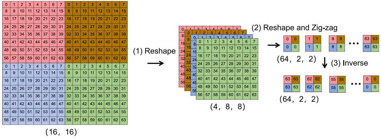
Fig. 2. Data Preprocessing. Taking a 16 \times 16 images as an example, four 8 \times 8 DCT blocks are processed according to frequency, zigzag scanning, and inverse ordering.
