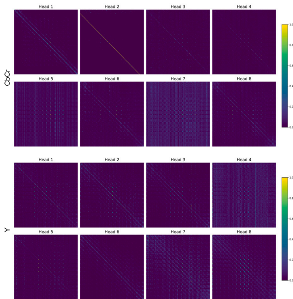
Fig. 7. Visualization of the learned self-attention maps from a transformer block in our context model. The top and bottom rows display the patterns for the 8 attention heads corresponding to the CbCr and Y channels, respectively. The diversity in patterns highlights the specialization of each head. For example, Head 2 (CbCr) approximates an identity function, while other heads focus on local or long-range spatial dependencies.
