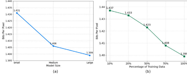
Fig. 6. Ablation studies on model scaling and data quantity. (a) Bits Per Pixel (BPP) for Small, Medium, and Large model variants, demonstrating the effectiveness of scaling model capacity. (b) The effect of training data volume on the Large model’s performance, showing a clear trend of improved compression with more data.
